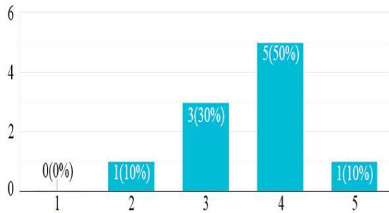
Figure 21 Evaluation case 6
