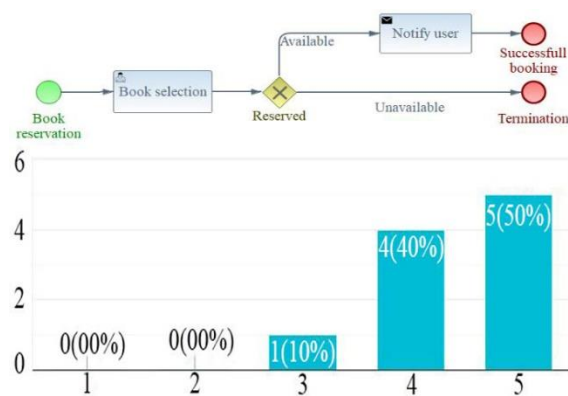
Figure 17 Evaluation case 2
