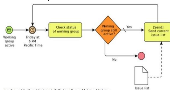
Figure 1 Example BPMN process
