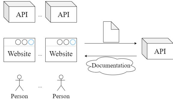
Figure 4 Application is available through both as a headless API and as human reachable Website.
