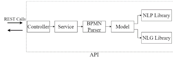
Figure 5 Internal application Architecture
