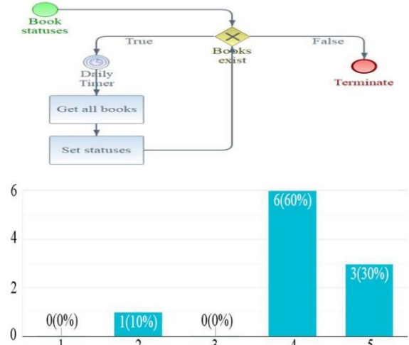
Figure 19 Evaluation case 4
