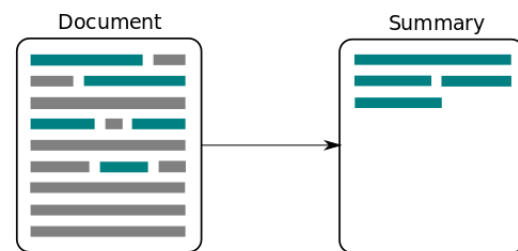
Figure 2 Text Summarization
