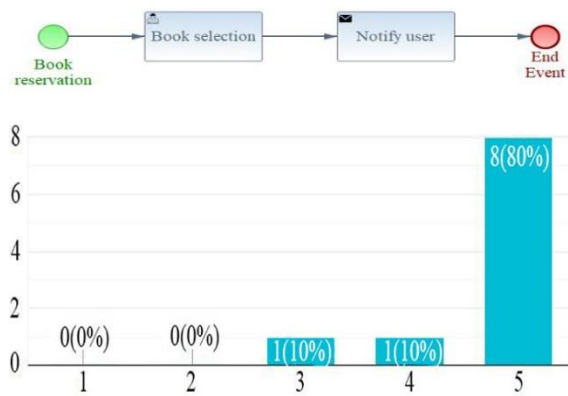
Figure 16 Evaluation case 1
