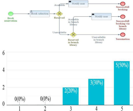
Figure 18 Evaluation case 3
