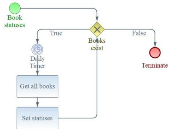
Figure 12 Example process with Timer Event
