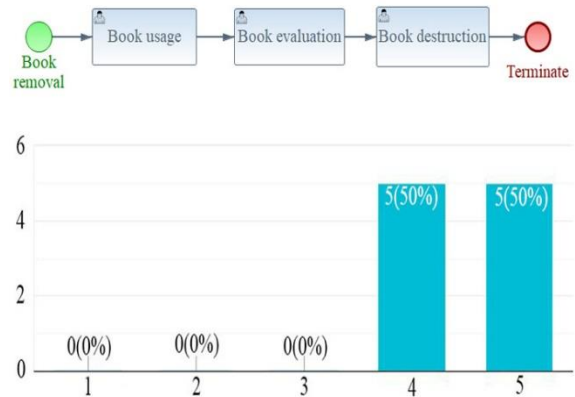
Figure 20 Evaluation case 5
