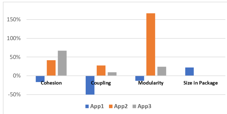
Figure 4: Application of DeRecGEA on Software Modularity
