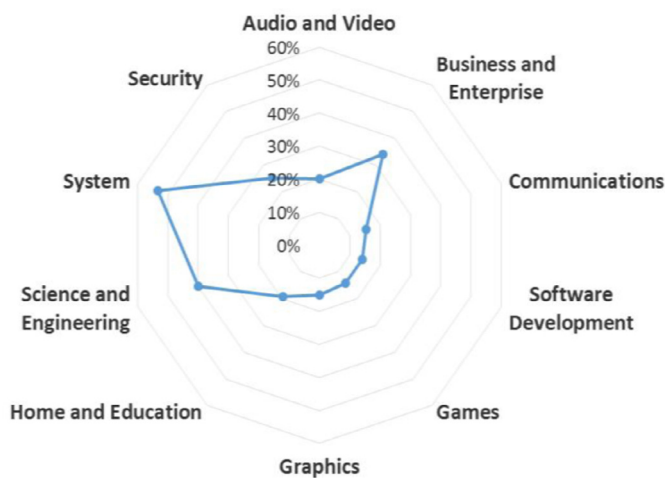
Fig. 5. Software maintainability.
