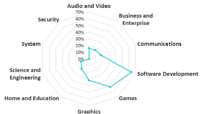
Fig. 4. Software adaptability.
