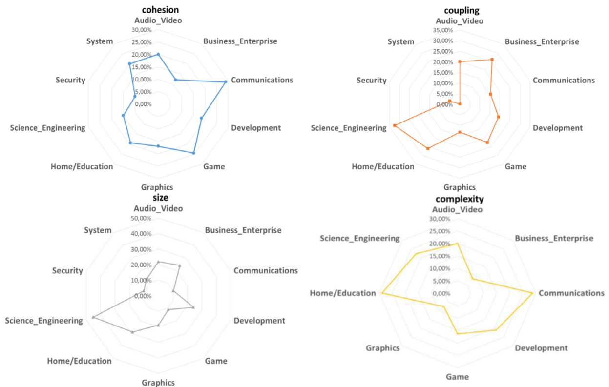
Fig. 9. Software complexity.
