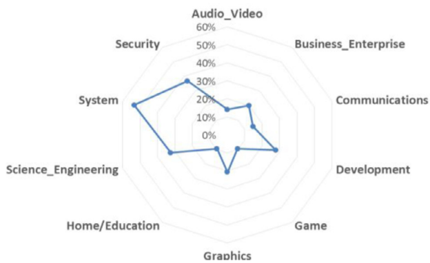
Fig. 7. Component availability.
