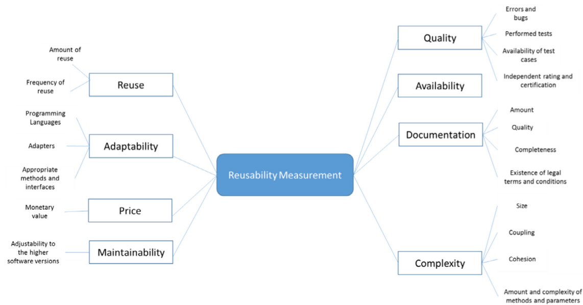
Fig. 2. Reusability measurement model.
