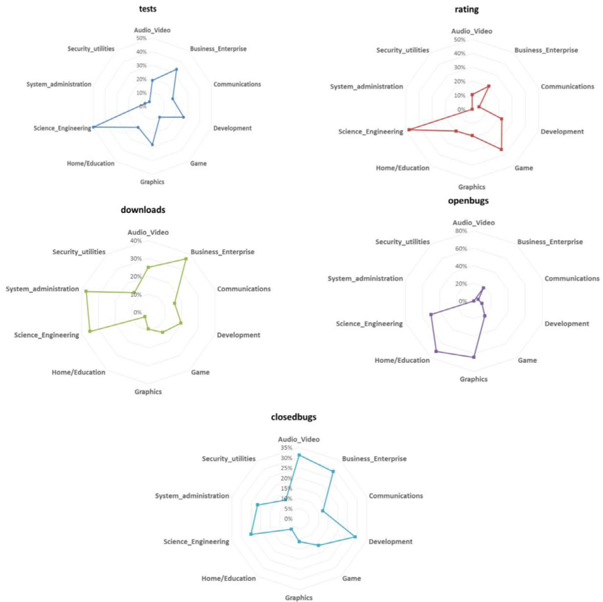
Fig. 6. Software external quality.
