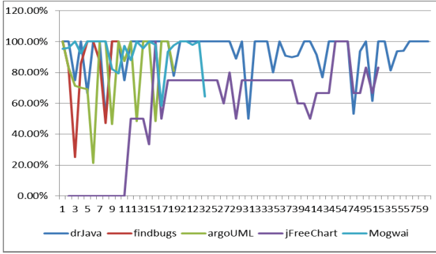
Figure 3. Evolution of the Number of Stable Libraries
